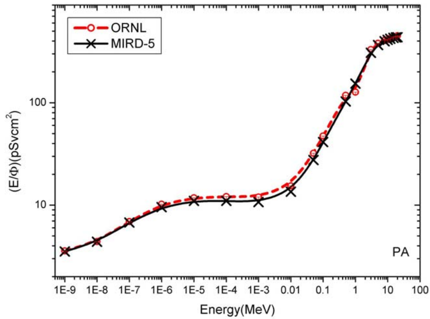
Figure 2. Effective doses per unit fluence for whole body in PA irradiation condition, according to ICRP60
