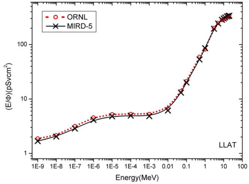
Figure 3. Effective doses per unit fluence for whole body in LLAT irradiation condition, according to ICRP60
