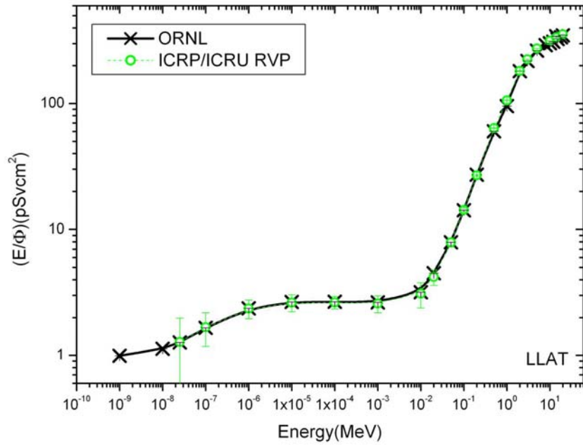
Figure 3. Effective doses per unit fluence for whole body in LLAT irradiation condition, according to ICRP103 .
