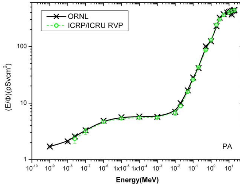
Figure 2. Effective doses per unit fluence for whole body in PA irradiation condition, according to ICRP103.
