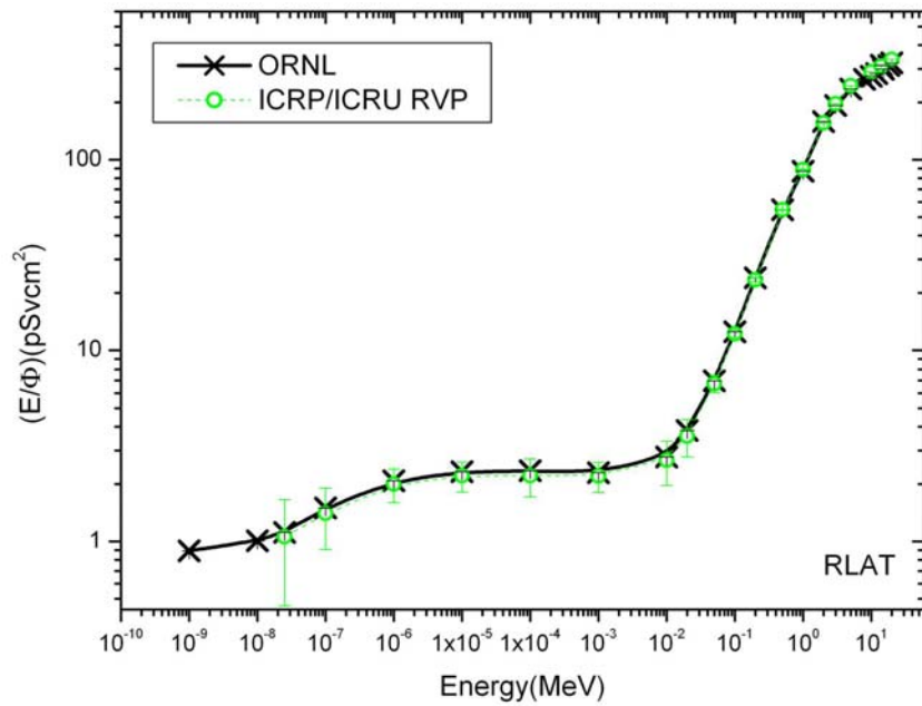
Figure 4. Effective doses per unit fluence for whole body in RLAT irradiation condition, according to ICRP103 .
