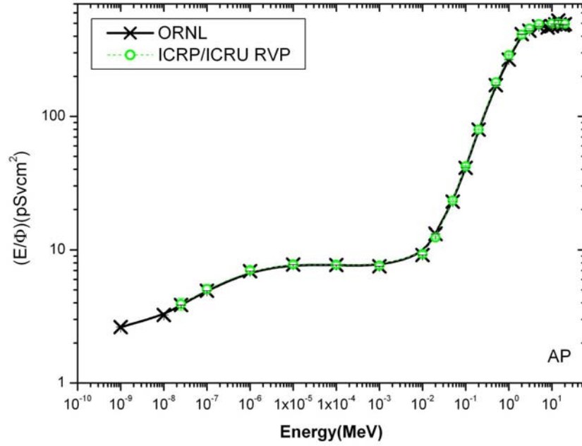
Figure 1. Effective doses per unit fluence for whole body in AP irradiation condition, according to ICRP103
