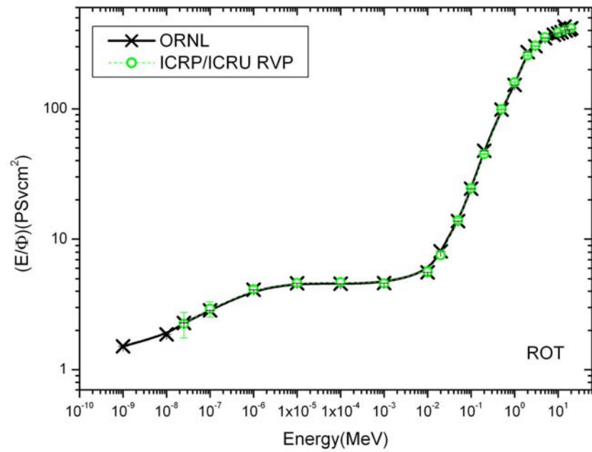
Figure 6. Effective doses per unit fluence for whole body in ROT irradiation condition, according to ICRP103 .
