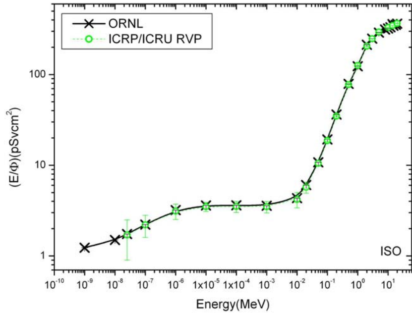
Figure 5. Effective doses per unit fluence for whole body in ISO irradiation condition, according to ICRP103 .
