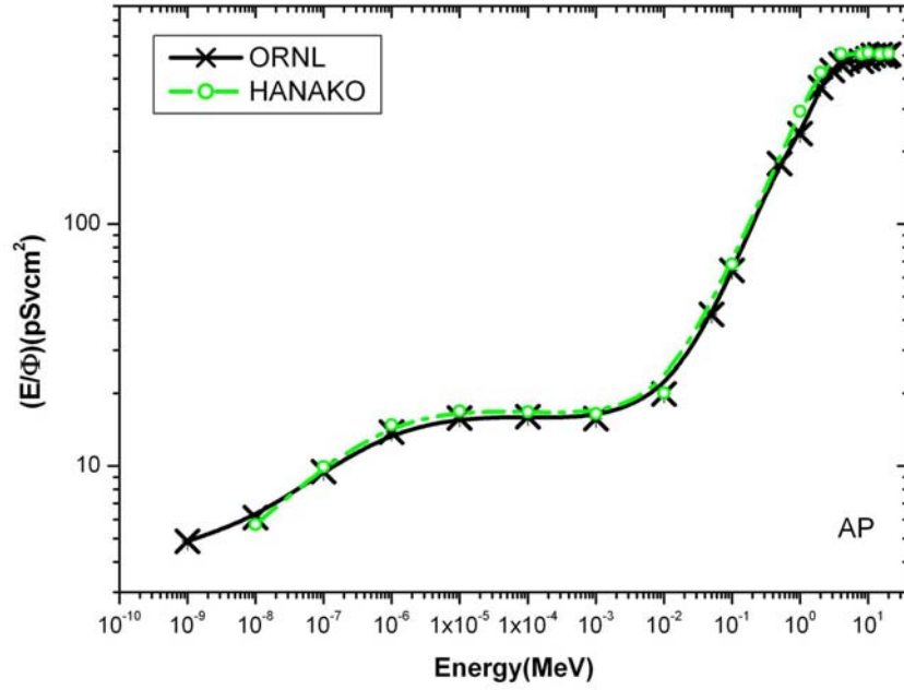
Figure 1. Effective doses per unit fluence for whole body in AP irradiation condition, according to ICRP60 .
