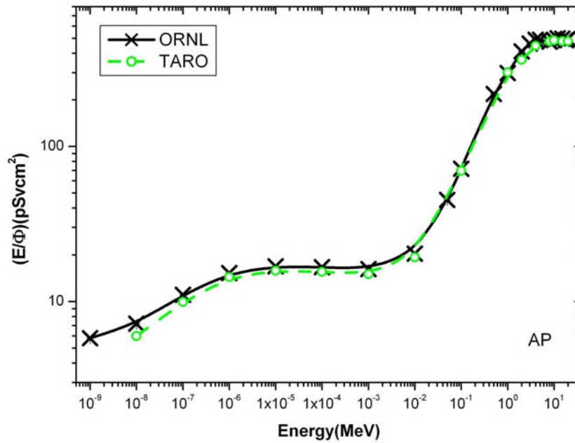
Figure 2. Effective doses per unit fluence for whole body in AP irradiation condition, according to ICRP60 .
